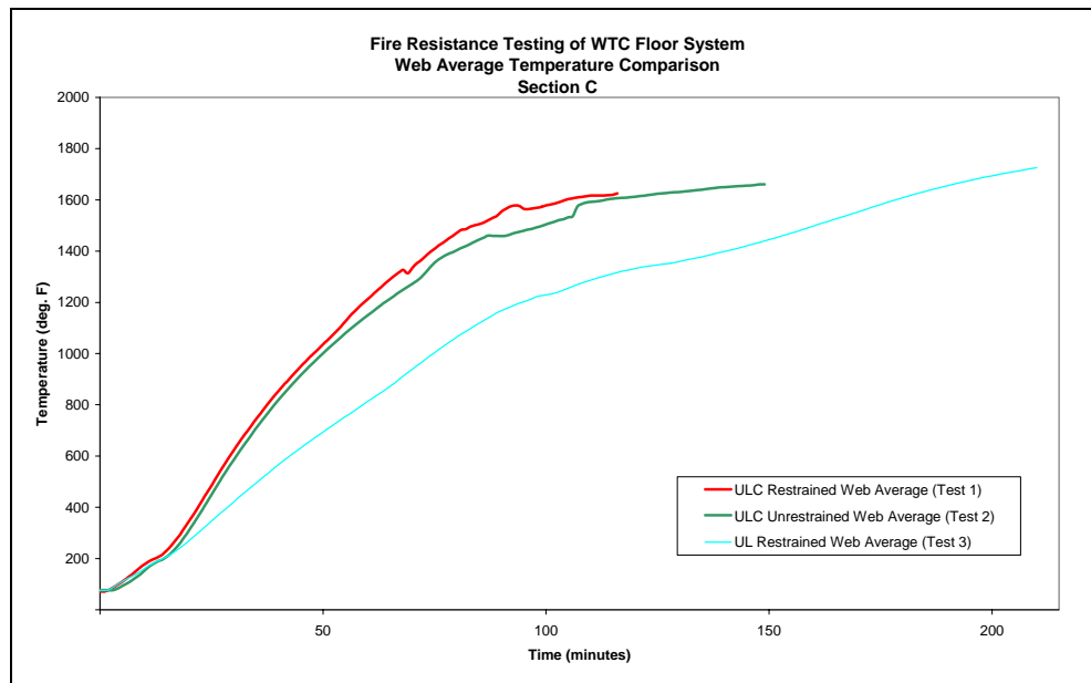
Figure 6–5. Average temperature of web diagonals for Test Nos. 1, 2, and 3 (3/4 in. thick SFRM).
