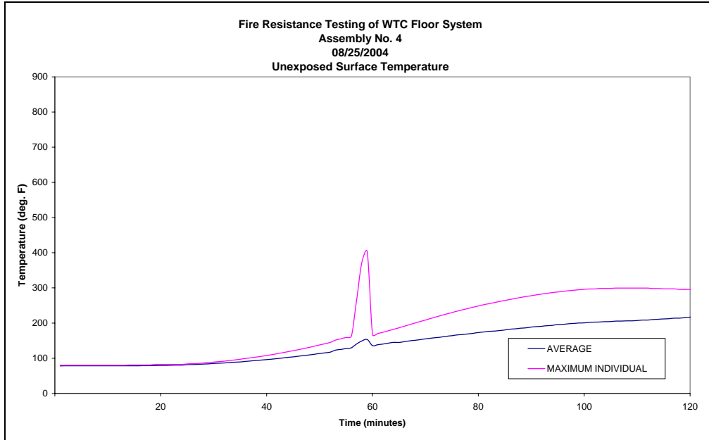
Figure 5–59. Assembly No. 4 – average and maximum individual temperatures on unexposed surface.
