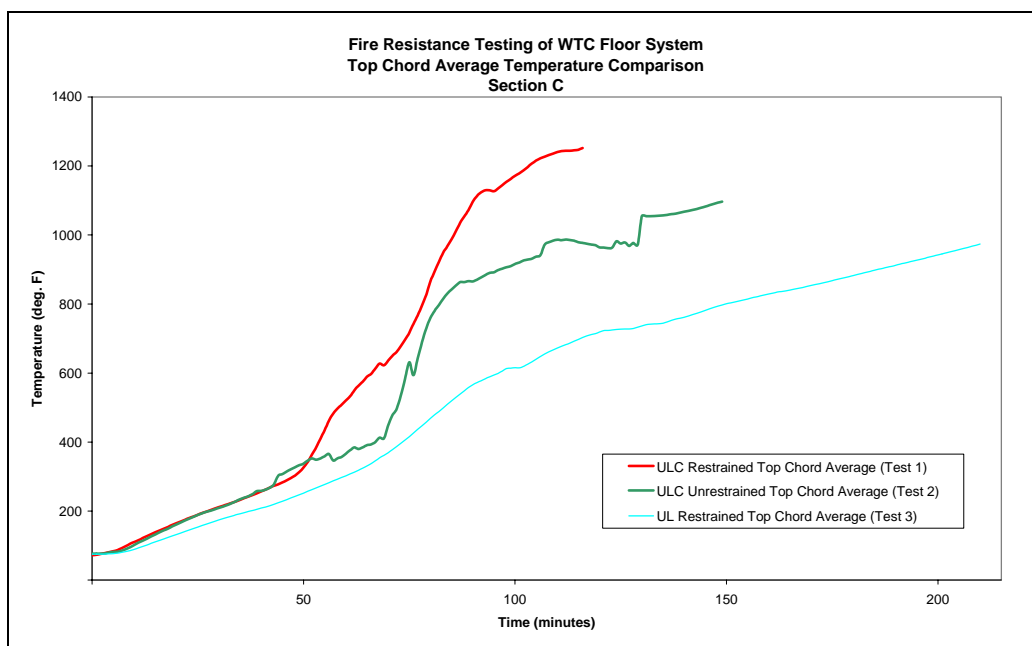
Figure 6–6. Average temperature of the top chord for Test Nos. 1, 2, and 3 (3/4 in. thick SFRM).
