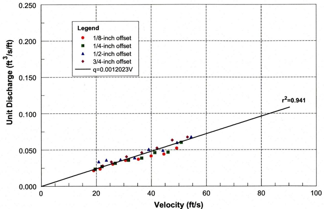
Figure VI-1-8 – Unit discharge for joint/crack, sharp-edged geometry, 1/2-inch gap.
