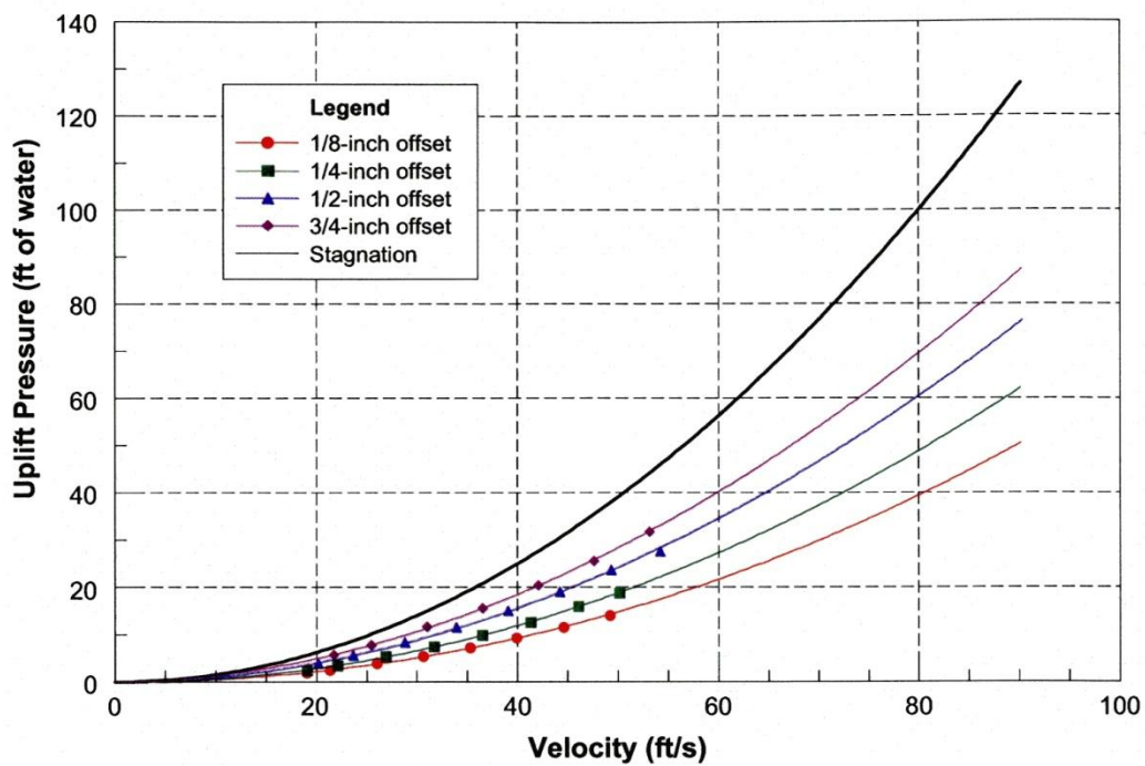
Figure VI-1-5 – Mean uplift pressure, sharp-edged geometry, vented cavity, 1/8-inch gap.
