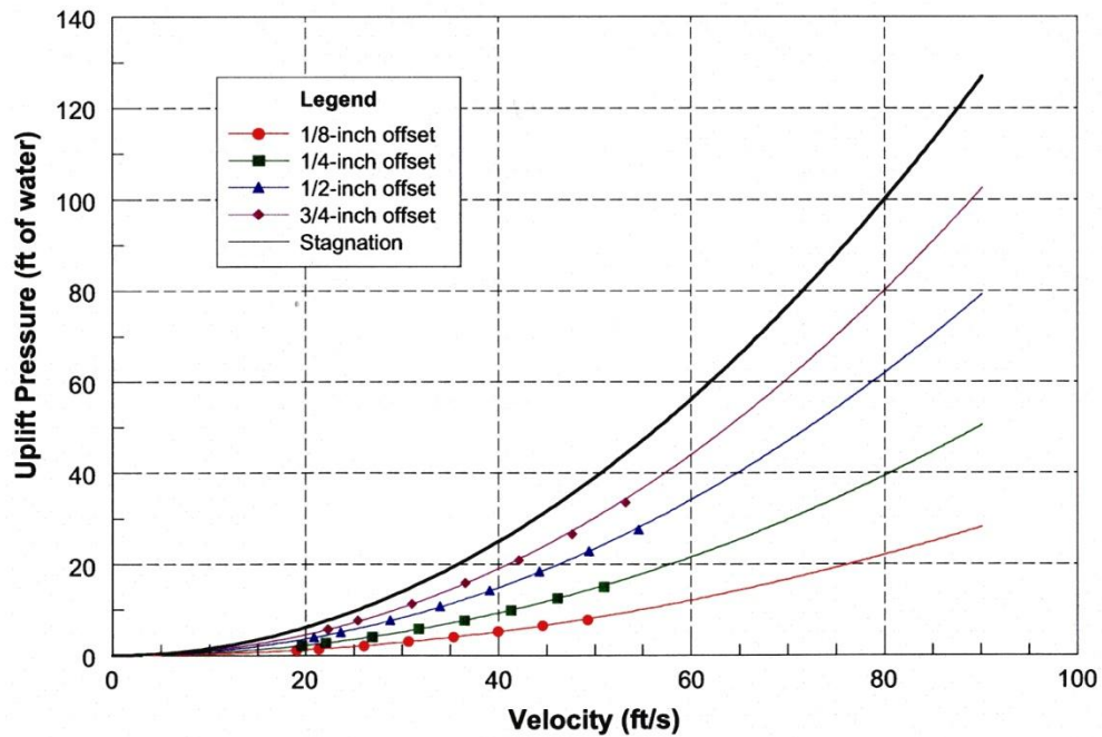
Figure VI-1-6 – Mean uplift pressure, sharp-edged geometry, vented cavity, 1/2-inch gap.
