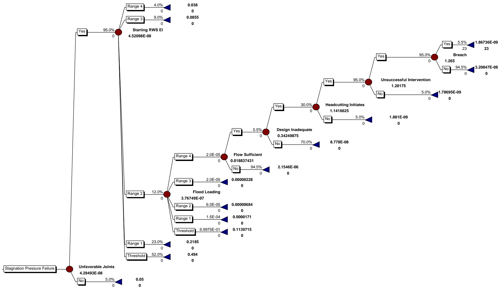
Figure VI-1-3 – Example Event Tree
