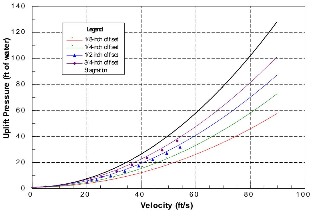
Figure VI-1-4 - Mean uplift pressure, sharp-edged geometry, sealed cavity, 1/8-inch gap.
