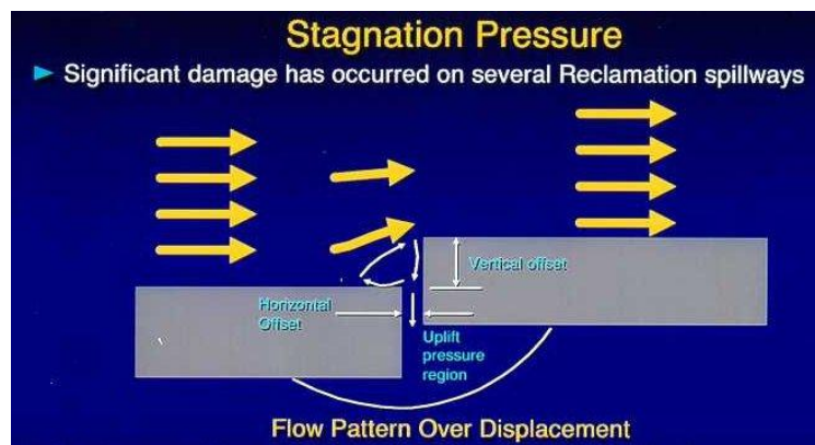
Figure VI-1-1 Stagnation Pressure Development
