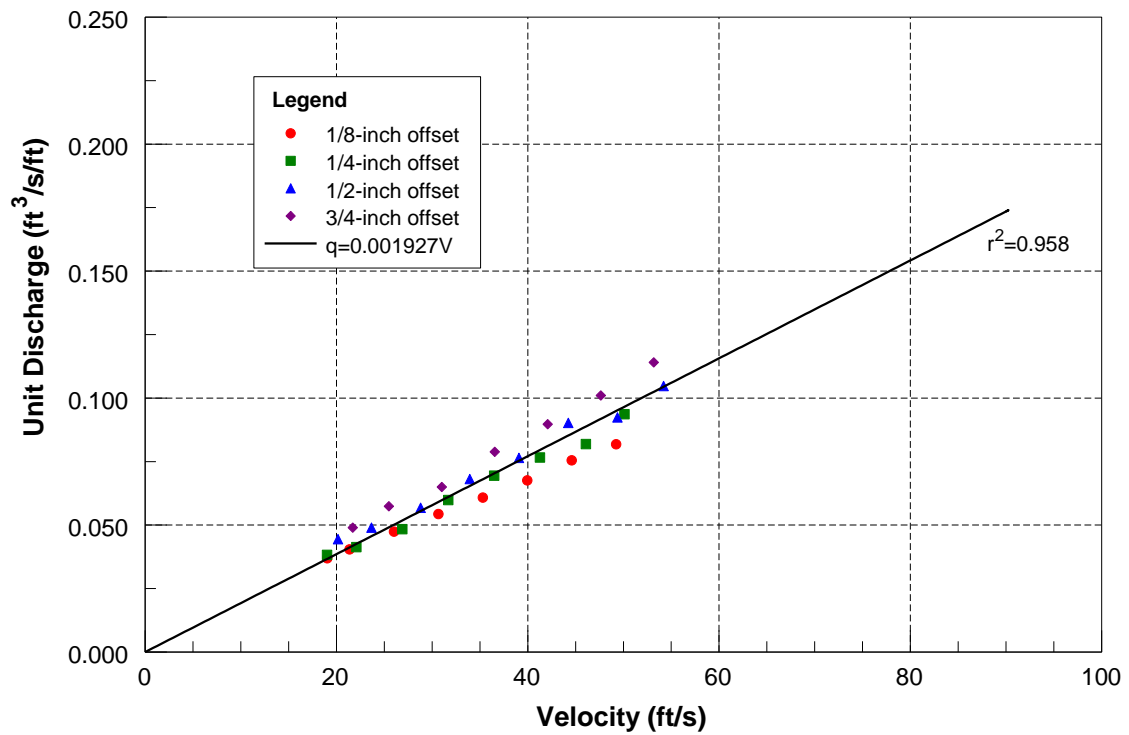
Figure VI-1-7 – Unit discharge for joint/crack, sharp-edged geometry, 1/8-inch gap.
