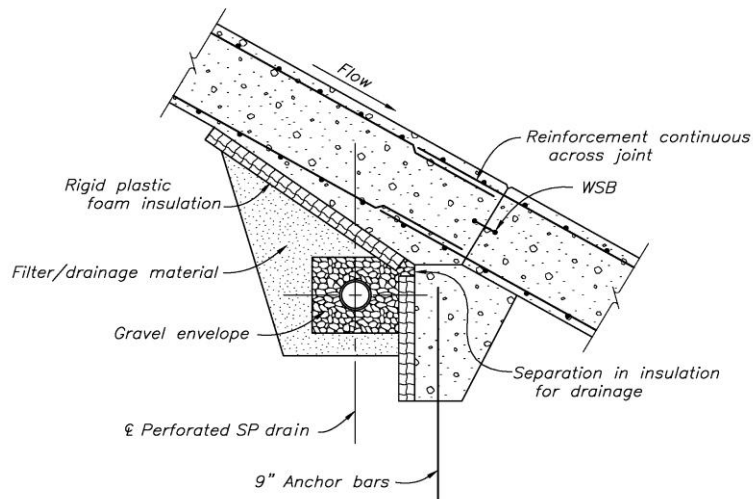
Figure VI-1-2 – Defensive Design Measures
