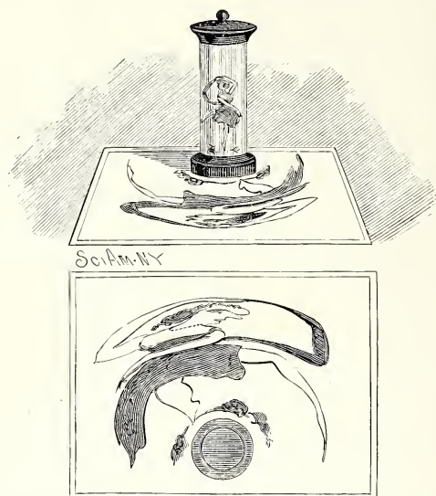
FIG. 8. ANAMORPHOSIS VIEWED IN CONVEX CYLINDRICAL MIRROR.*
