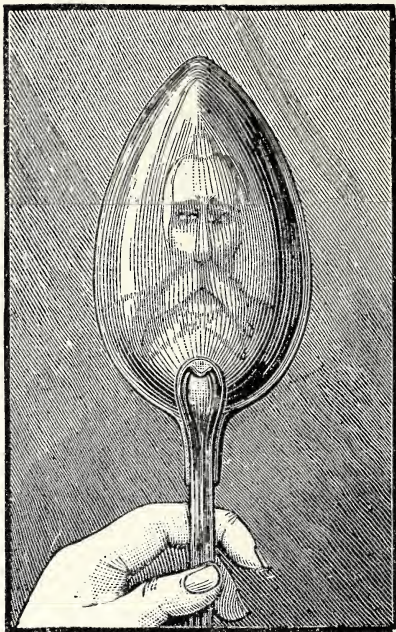
FIG. 6.—ELONGATED REFLECTION IN A SPOON.
