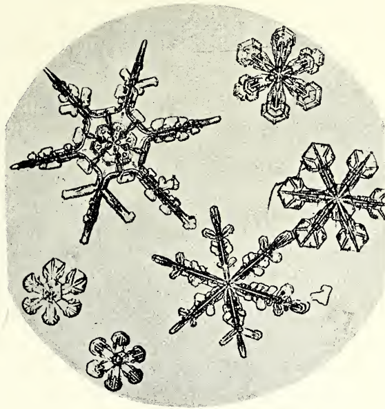
FIG. 62. SNOW CRYSTALS. PHOTO BY DR. NEUHAUS.
